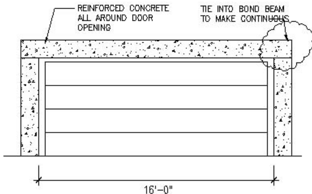
TYPICAL SINGLE FAMILY HOME GARAGE DOOR (ALT 1) N.T.S.
