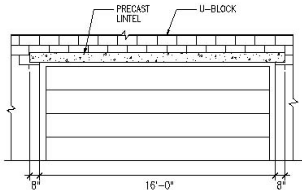
TYPICAL SINGLE FAMILY HOME GARAGE DOOR (ALT 2) N.T.S.
