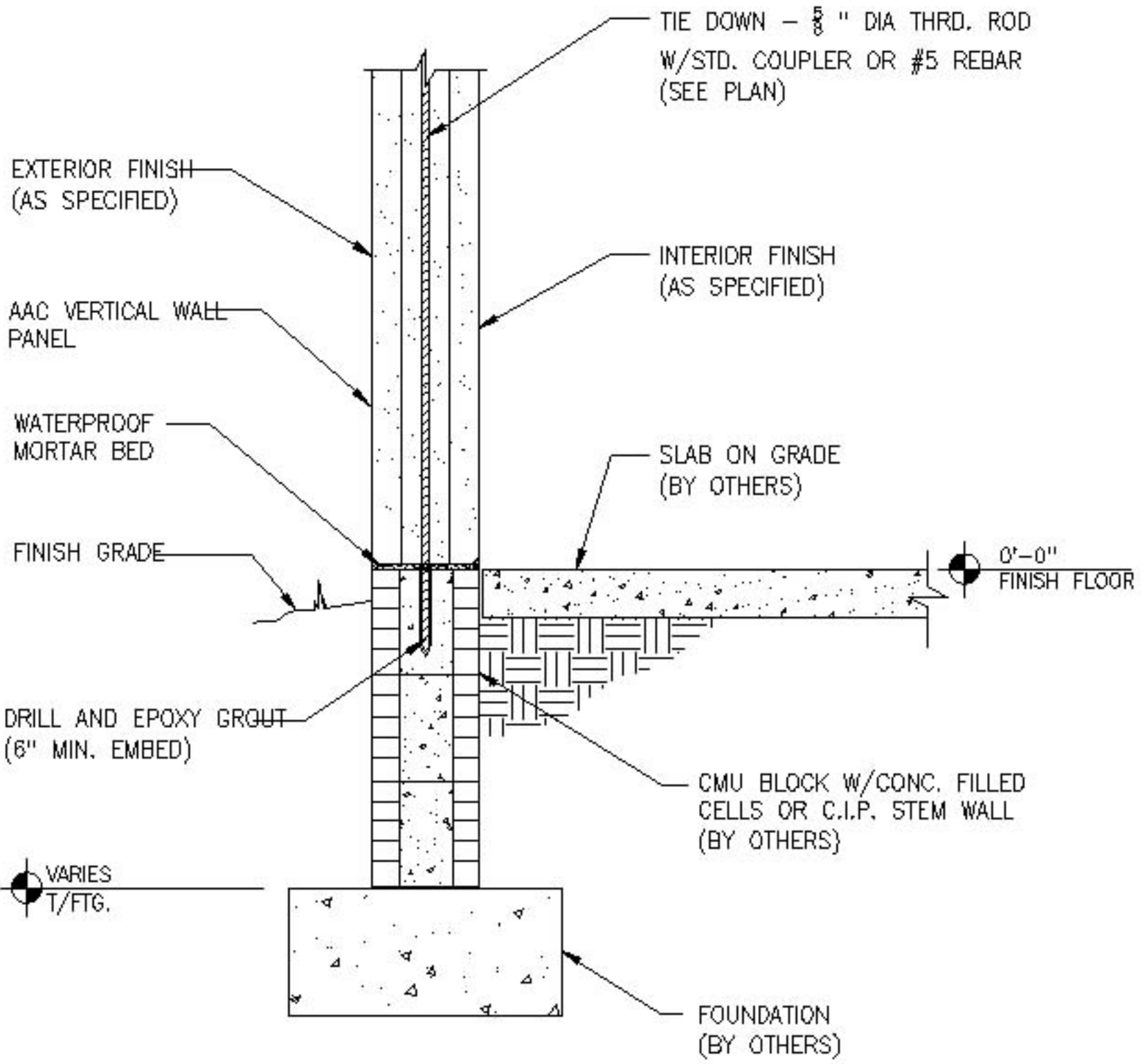
FLOOR PANEL @ CMU WALL 1" = 1'-0"
