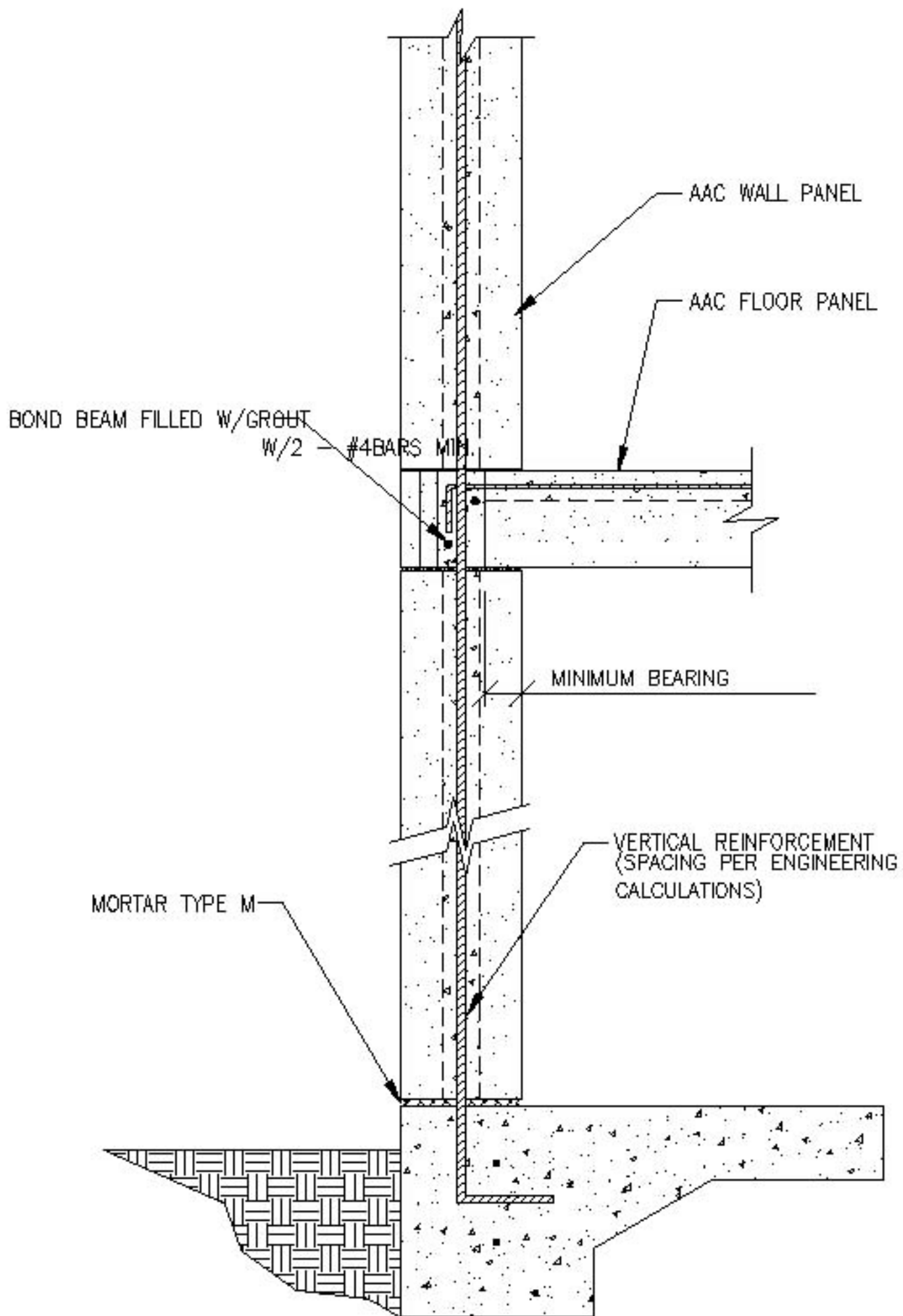
VERTICAL WALL PANEL @ EXTERIOR WALL 1" = 1'-0"
