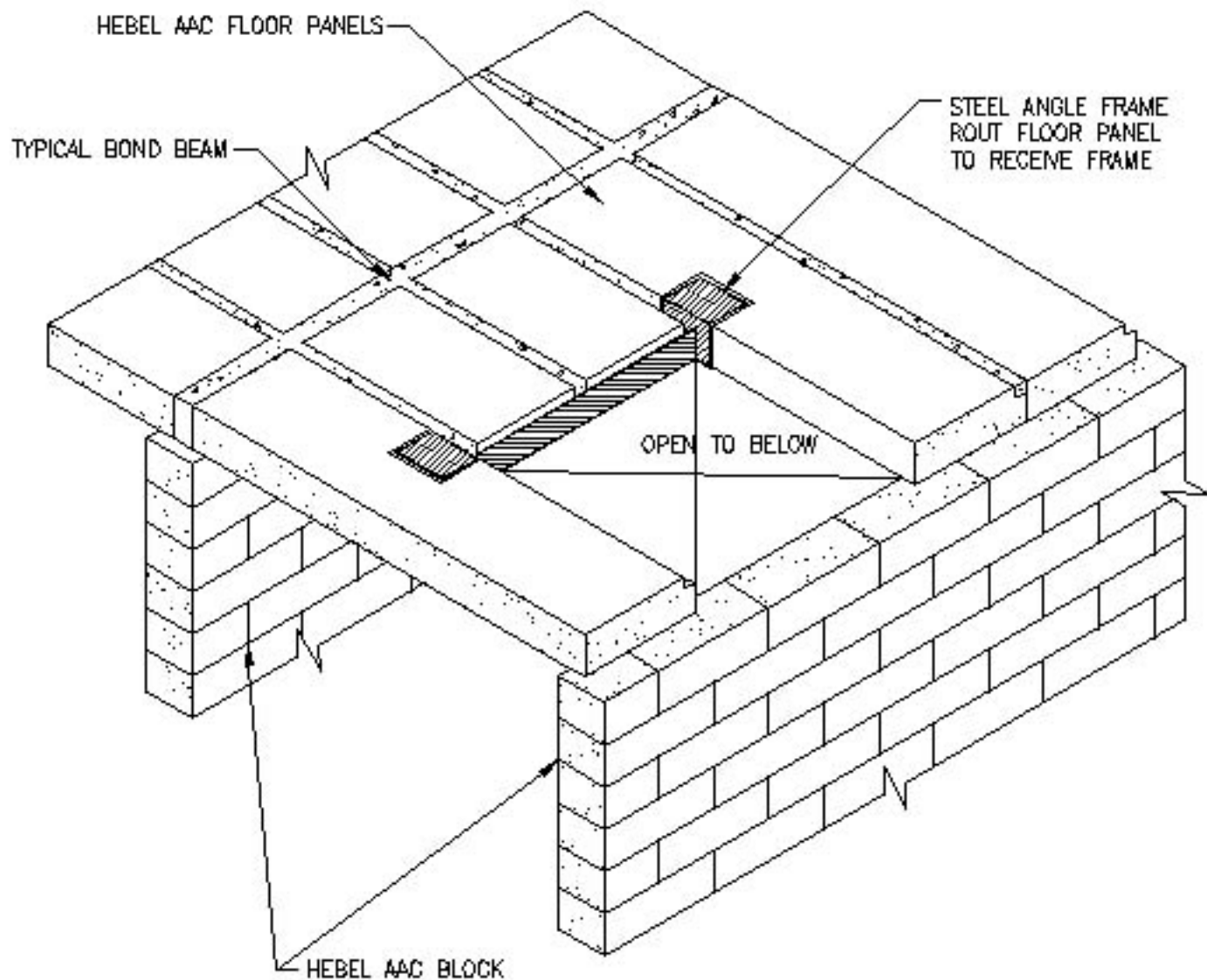
7 TYPICAL CHASE OPENING HX 3/4"=1'-0" (AT END OF PANEL SPAN)
