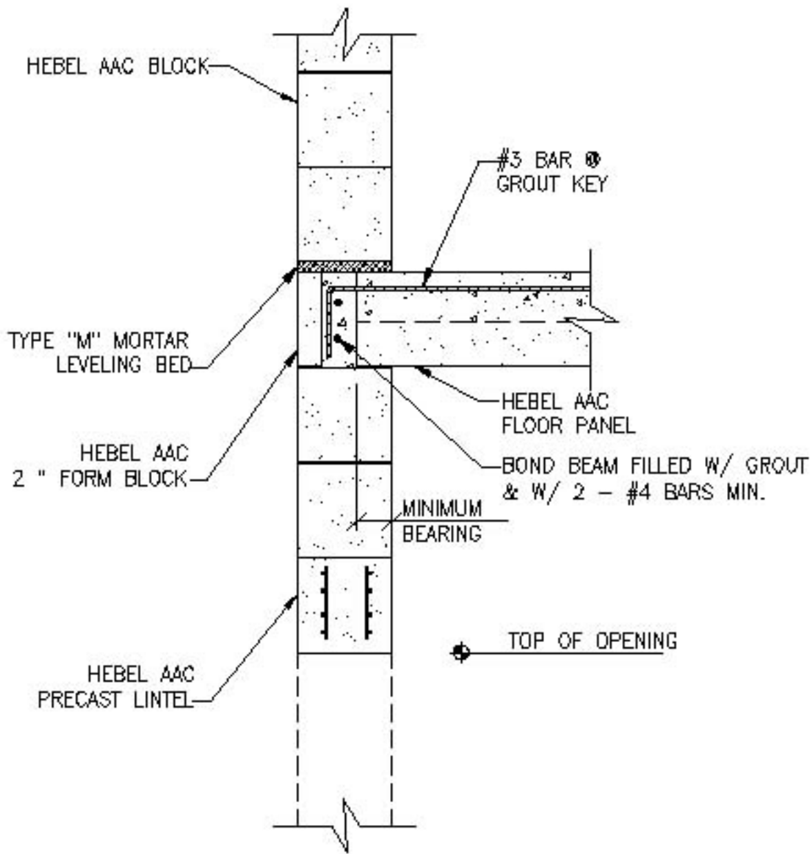
WALL SECTION @ FLOOR ABOVE OPENING
