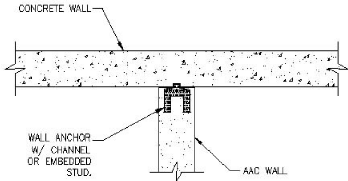
AAC WALL - CONCRETE WALL CONNECTION 1" = 1'-0"
