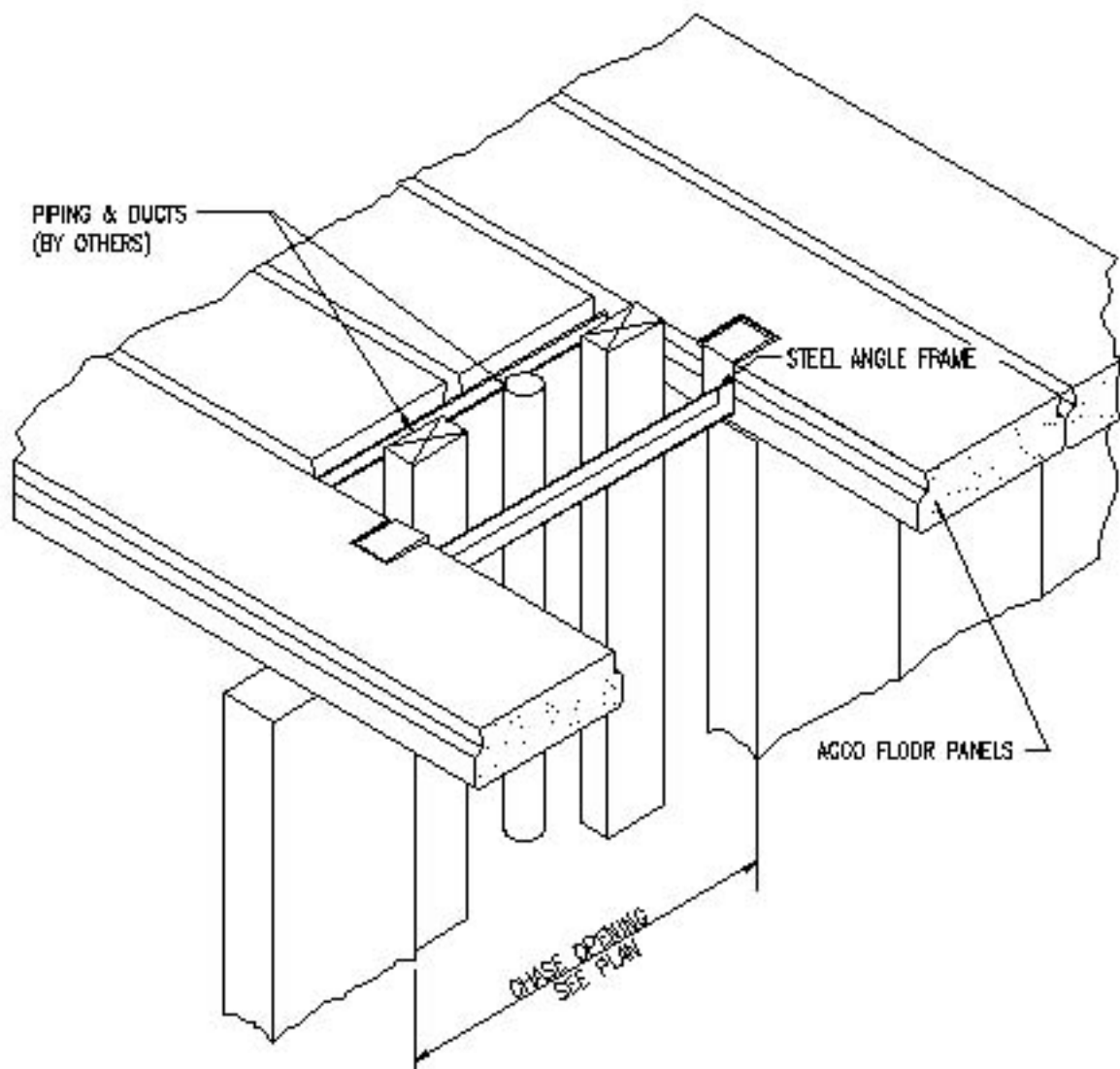
CHASE OPNG W/ PANEL SUPPORT
