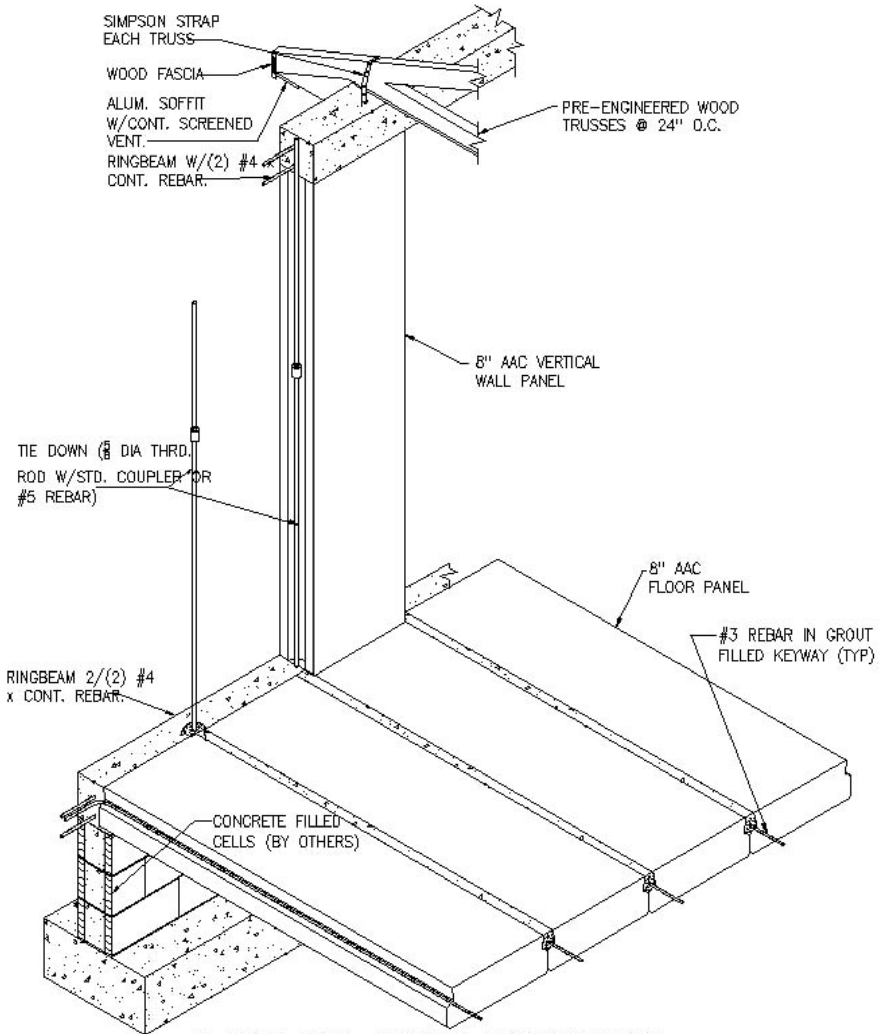
FLOOR AND TRUSS CONNECTION N.T.S.
